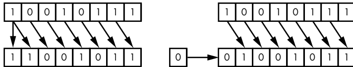
Figure 4-2: Arithmetic (signed) right shift and logical (unsigned) right shift of 1 bit
