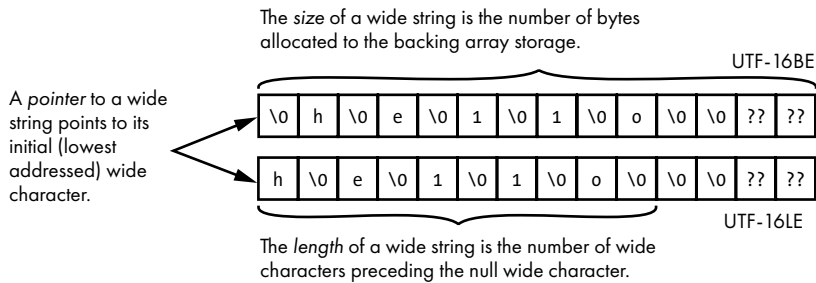
Figure 7-2: Sample UTF-16LE wide string
