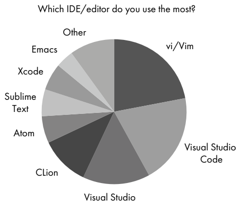
Figure 1-1: IDE/editor use
