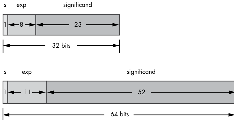
Figure 3-2: The float and double types
