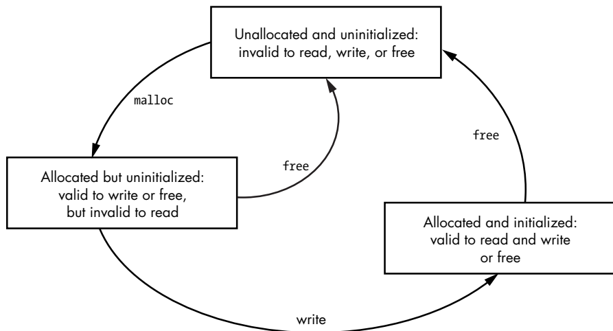
Figure 6-1: Memory states
