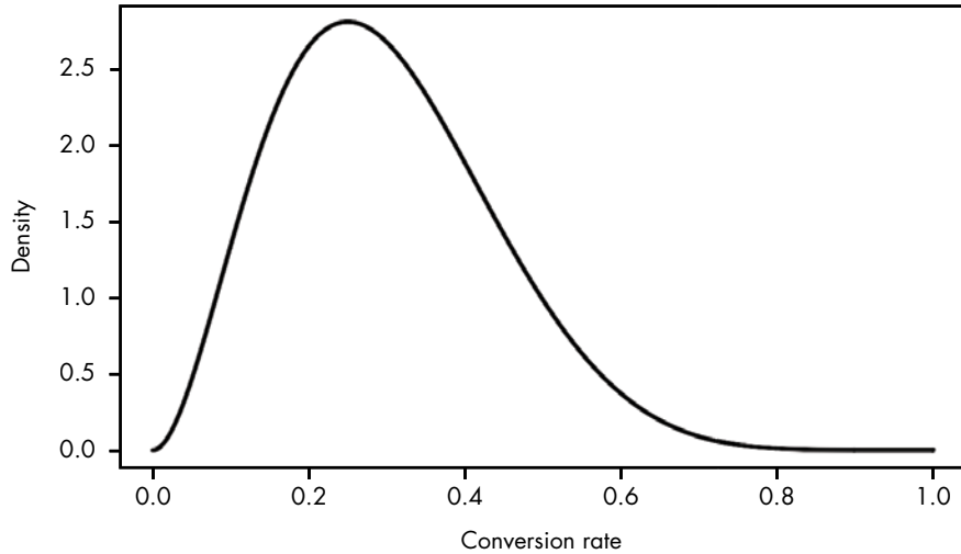
Figure 15-1: Visualizing our prior probability distribution
