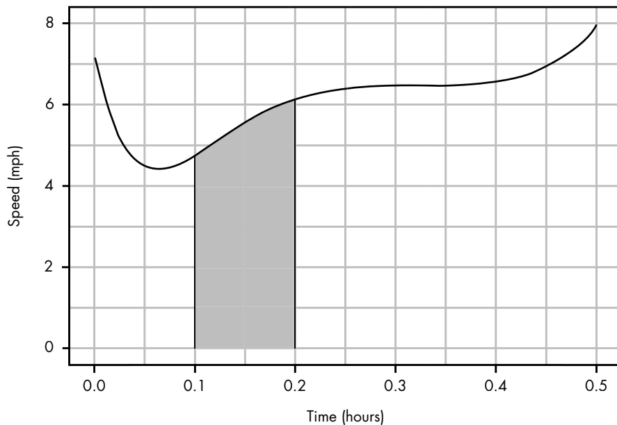
Figure B-7: Visualizing the area under the curve for the region from 0.1 to 0.2
