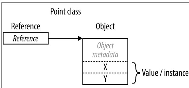
Figure 3. A reference type instance in memory
