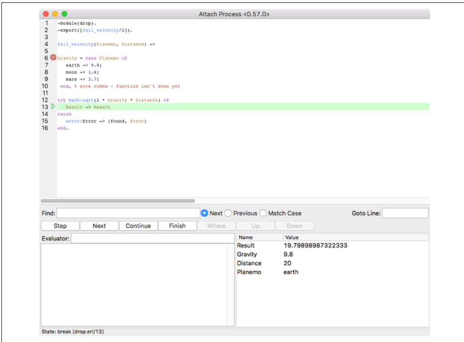
Figure 9-11. A successful calculation leads to line 13, which provides the return value
