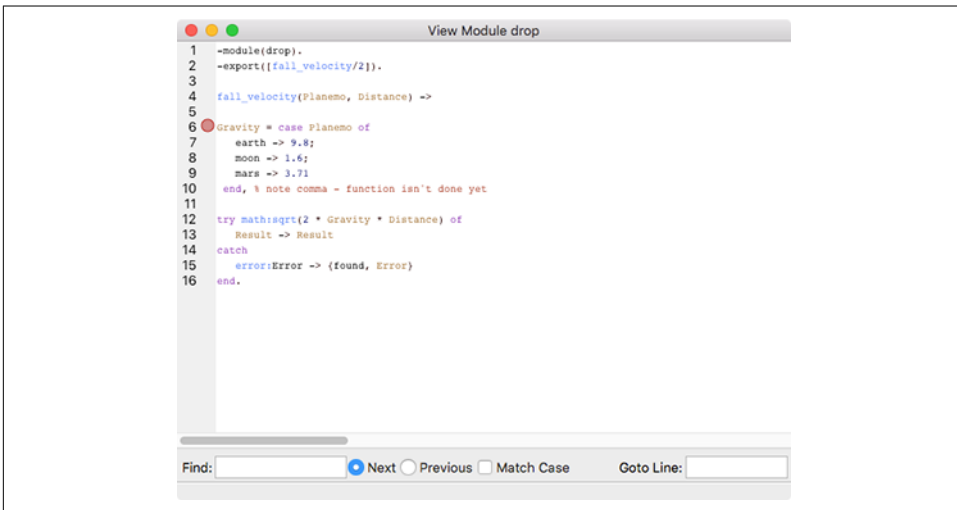
Figure 9-6. The drop module with a breakpoint set on line 6
