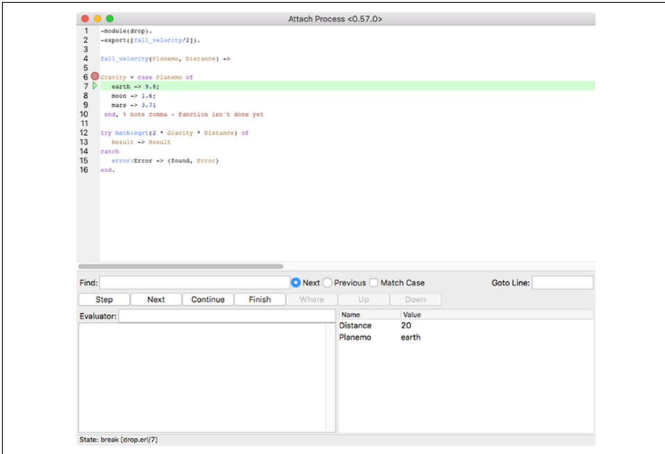
Figure 9-9. Stepping to the match on line 7
