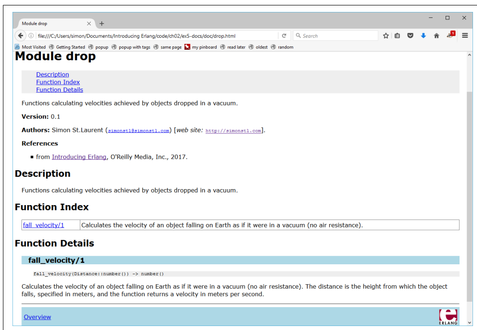
Figure 2-3. EDoc documentation with type information
