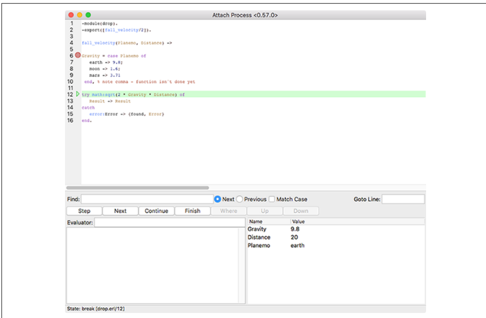
Figure 9-10. Next step: the try statement and calculation on line 12, with additional bound values
