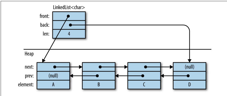
Figure 16-4. A LinkedList<char> in memory
