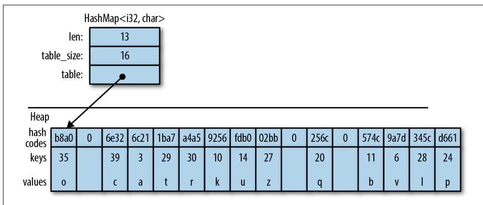
Figure 16-5. A HashMap in memory
