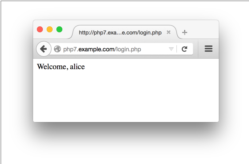
Figure 10-5. Successful login
