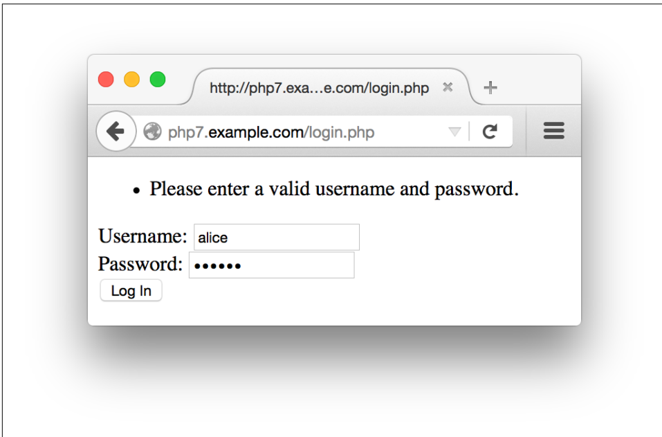
Figure 10-4. Unsuccessful login
