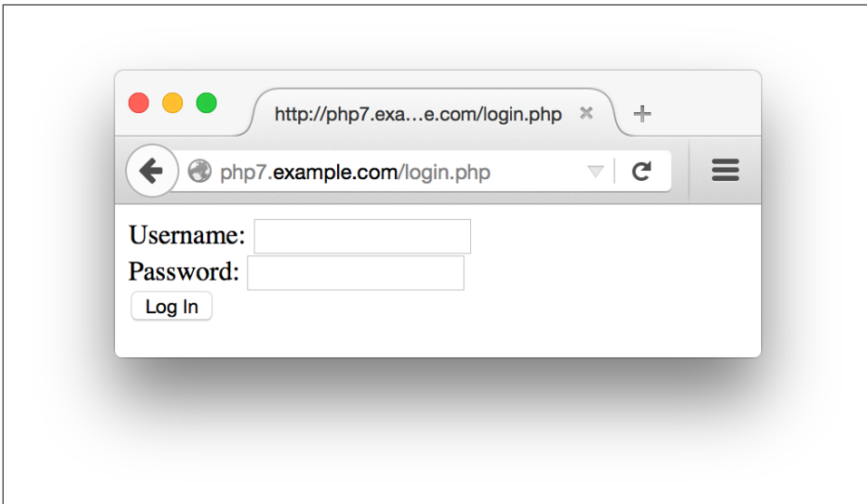
Figure 10-3. Login form
