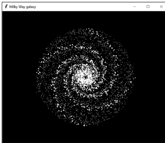
Figure 10-9: The Milky Way, modeled using logarithmic spirals
