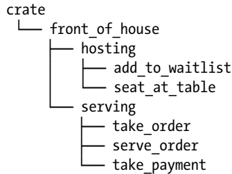
Listing 7-2: The module tree for the code in Listing 7-1
