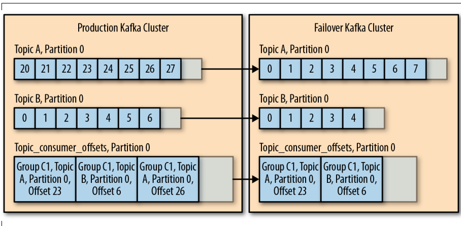
Figure 8-5. A fail over causes committed offsets without matching records
