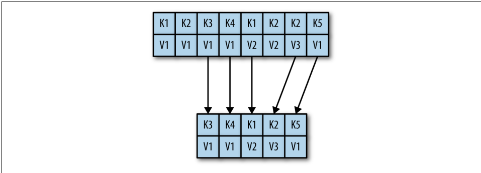
Figure 5-8. Partition segment before and after compaction
