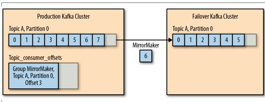
Figure 8-7. Monitoring the lag difference in offsets
