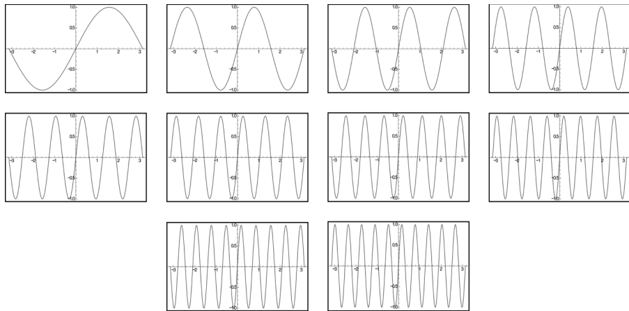
FIGURE BC-3: Ten plots with increasing frequency in each.
