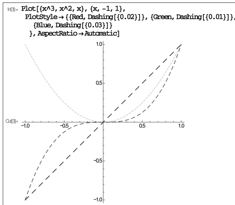
FIGURE BC-5: Three powers of x .
