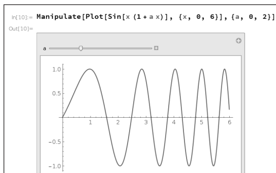
FIGURE BC-4: A manipulate slider.
