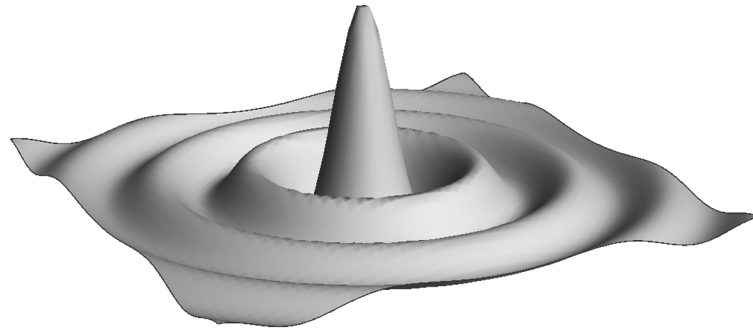
FIGURE BC-11: A sinc function.
