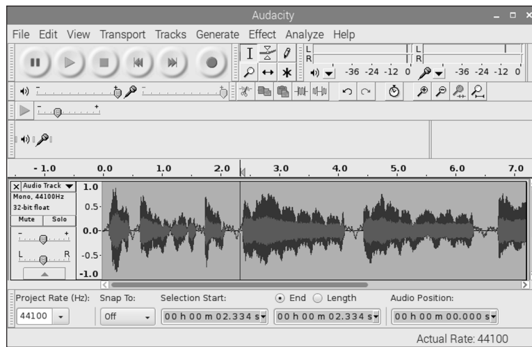
FIGURE 18-6: Audacity.
