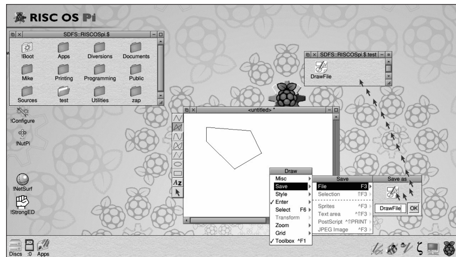
FIGURE C-3: !Draw saving.
