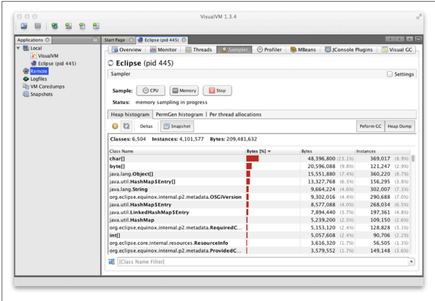
Figure A-5. Sampler tab
