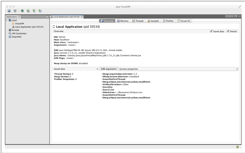
Figure A-2. Overview tab
