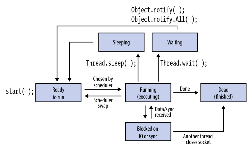
Figure 6-4. Thread lifecycle
