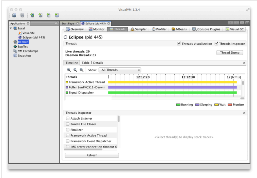
Figure A-4. Threads tab
