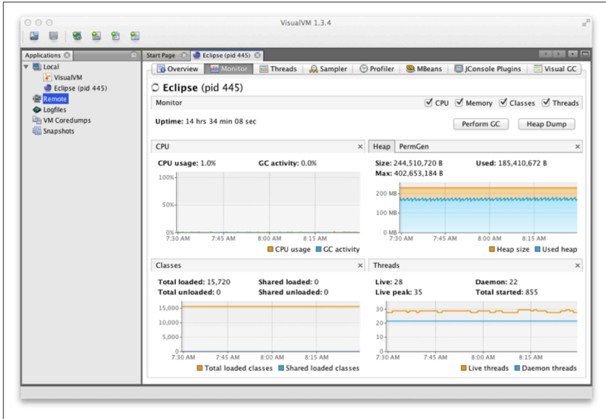
Figure A-3. Monitor tab
