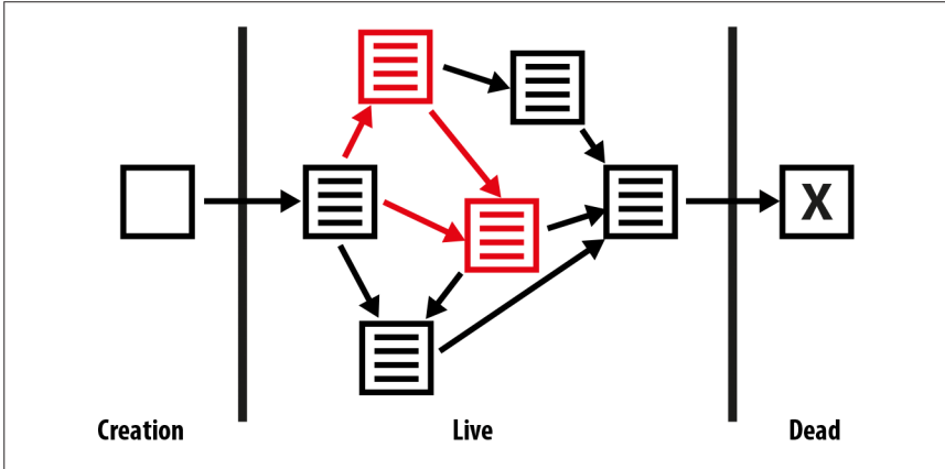
Figure 5-1. Program state transitions
