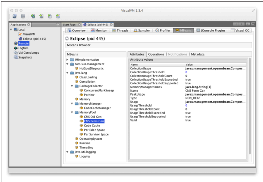
Figure A-6. MBeans plug-in
