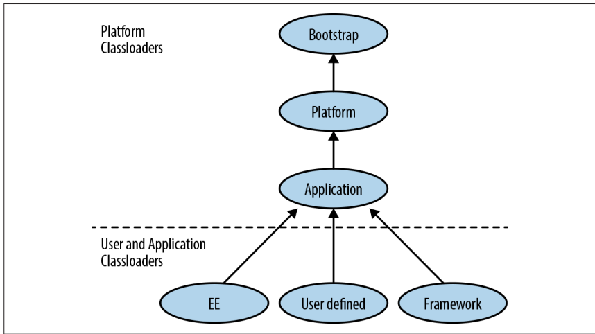
Figure 11-2. Classloader hierarchy
