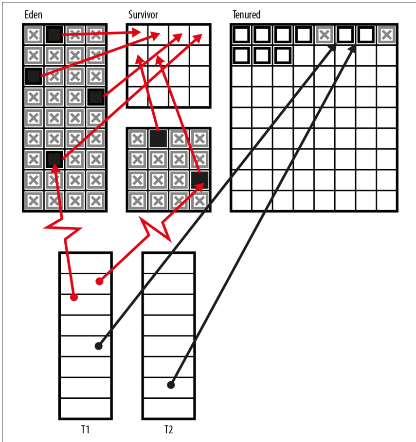
Figure 6-1. Heap structure
