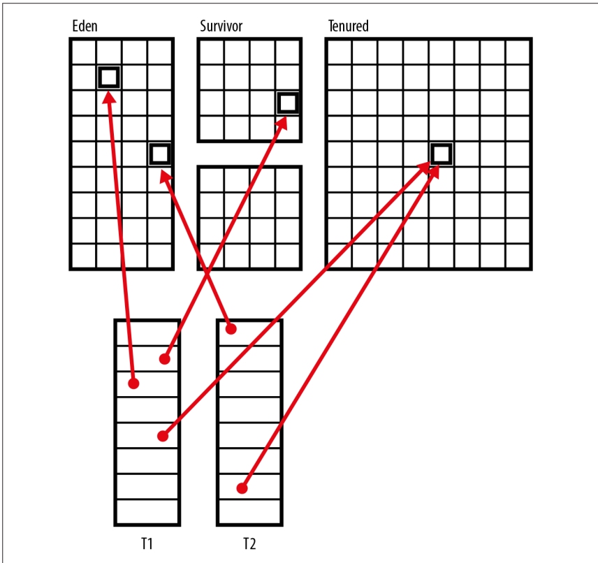
Figure 6-5. Shared memory between threads
