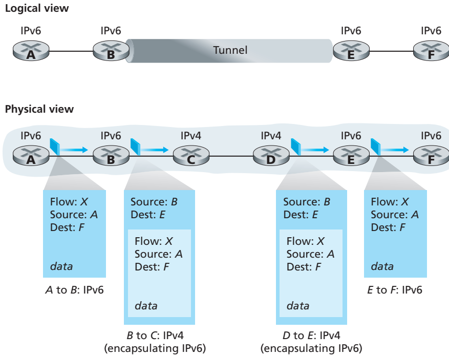
Figure 4.27 ♦ Tunneling
