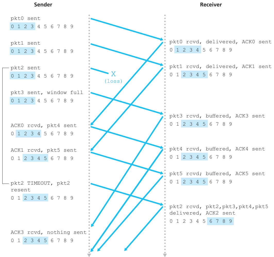
Figure 3.26 ♦ SR operation
