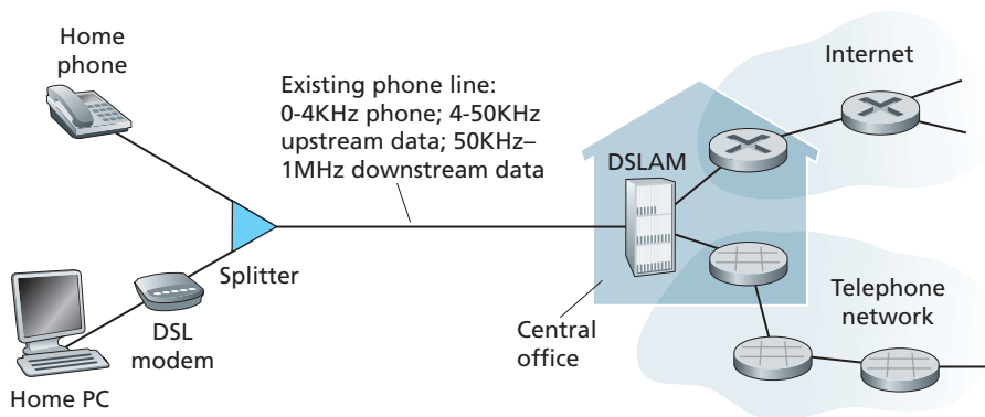
Figure 1.5 ♦ DSL Internet access
