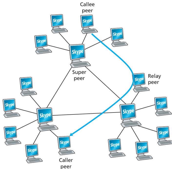
Figure 9.7 ♦ Skype peers
