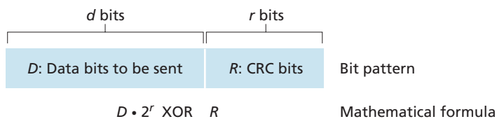
Figure 6.6 ♦ CRC
