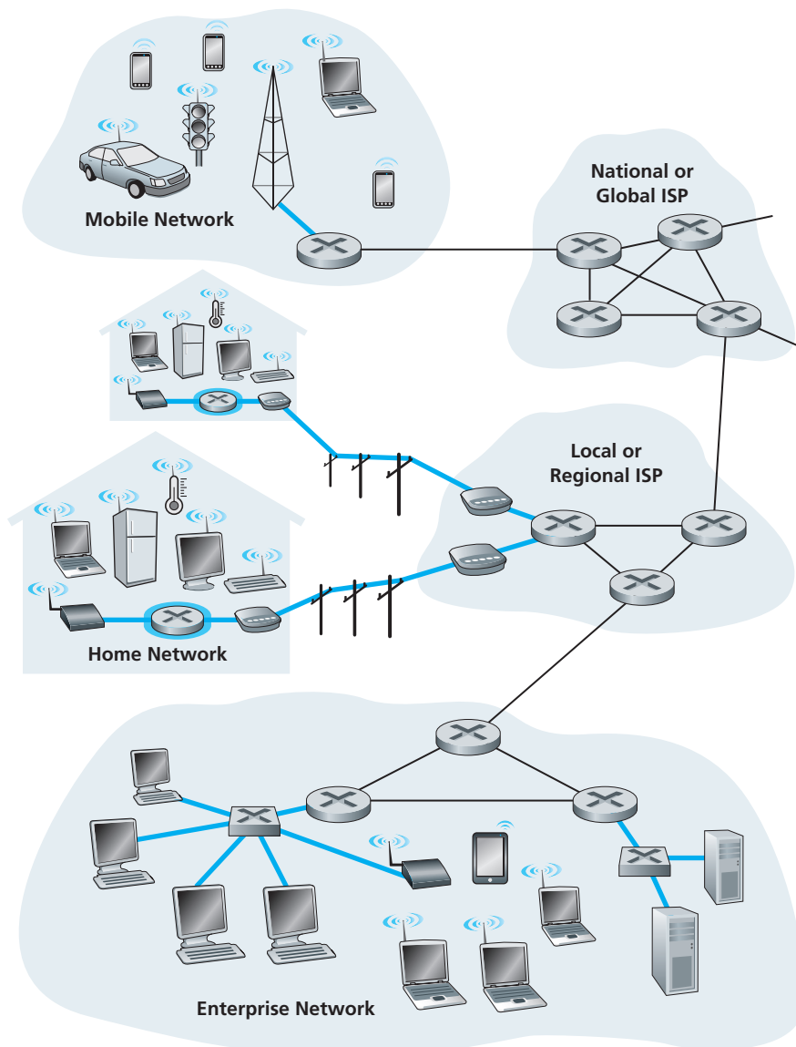
Figure 1.4 ♦ Access networks
