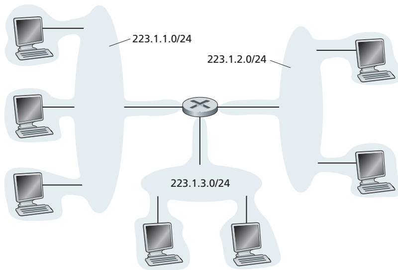
Figure 4.19 ♦ Subnet addresses
