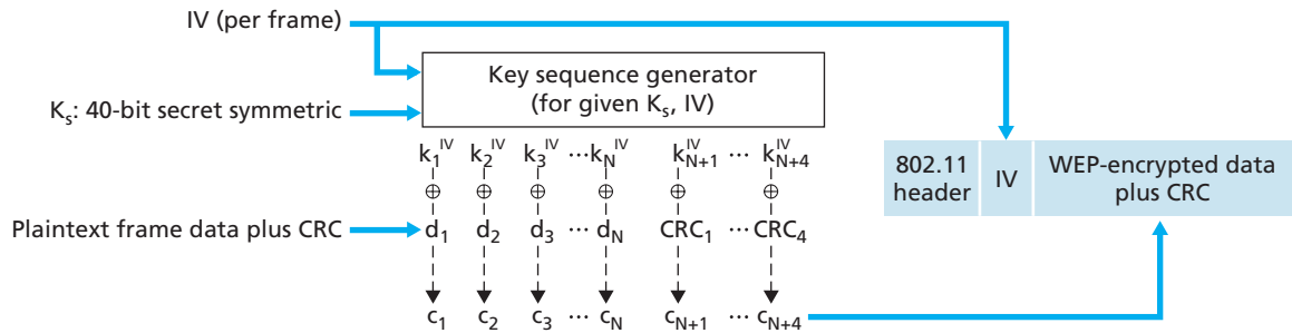
Figure 8.30 ♦ 802.11 WEP protocol
