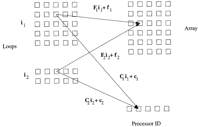
Figure 11.25: Space-partition constraints
