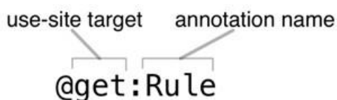
Figure 10.1 The syntax for specifying use-site targets
