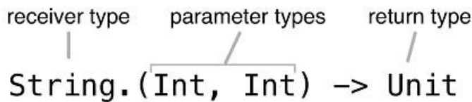
Figure 11.1 An extension function type with receiver type 'String' and two parameters of type 'Int', returning 'Unit'
