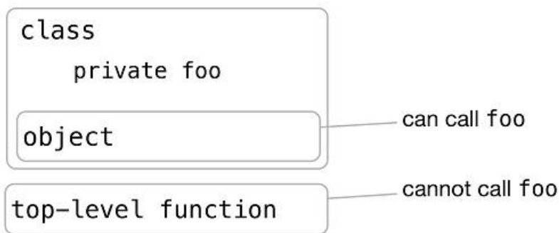
Figure 4.5 Private members can't be used in top-level util functions outside of the class
