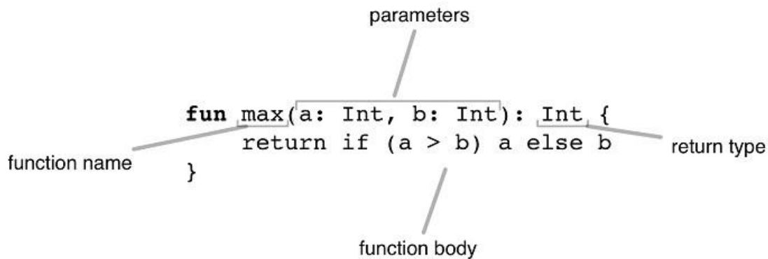
Figure 2.1 Kotlin function declaration
