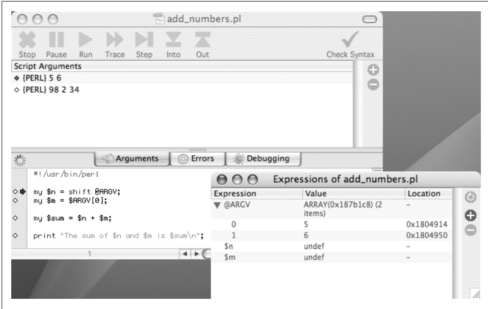
Figure 4-6. Affrus allows me to configure several different command lines to use with my program; it updates expressions as my program runs
