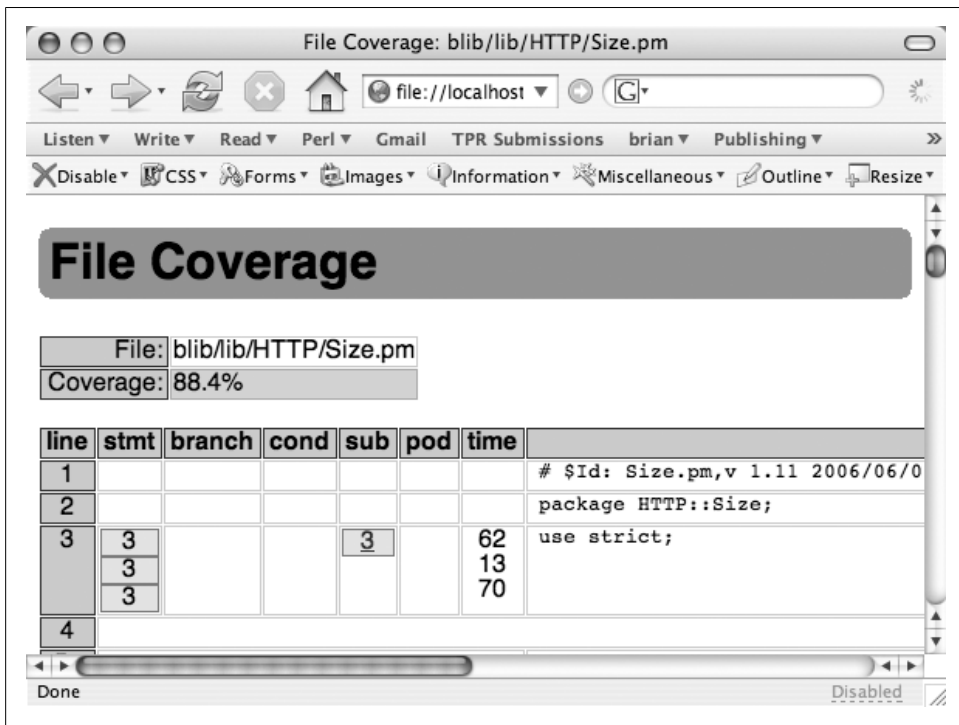
Figure 5-2. The coverage report for a particular file shows me how well I tested that line of code measurement on that line of code, and red to tell me that I have more testing work to do (Figure 5-2).
