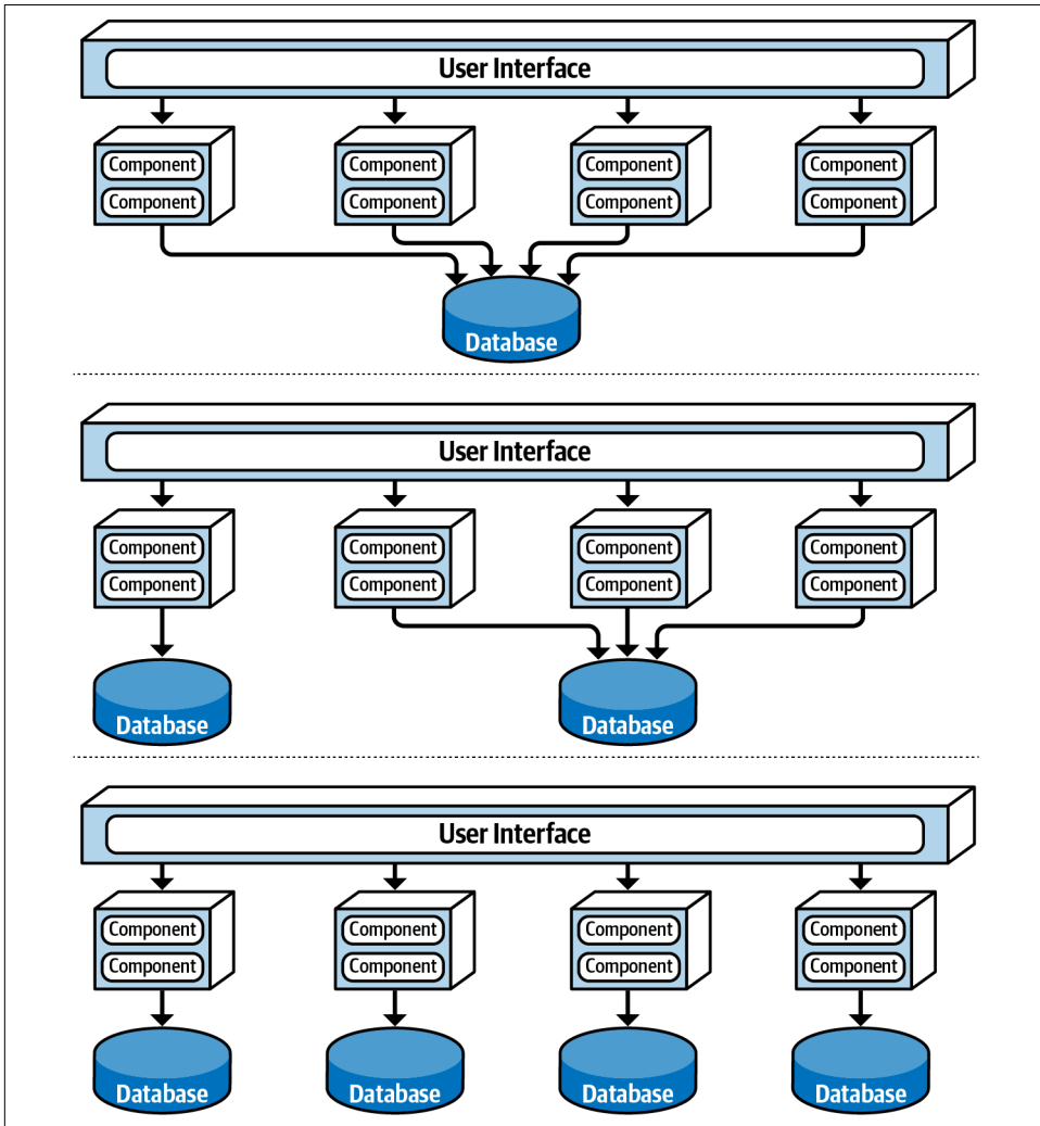
Figure 13-3. Database variants
