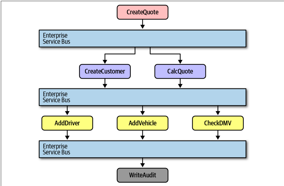
Figure 16-2. Message flow with service-oriented architecture
