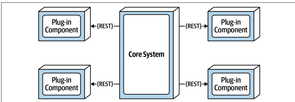
Figure 12-6. Remote plug-in access using REST
