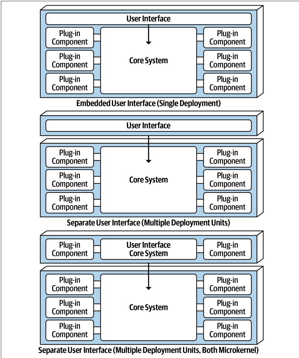
Figure 12-3. User interface variants
