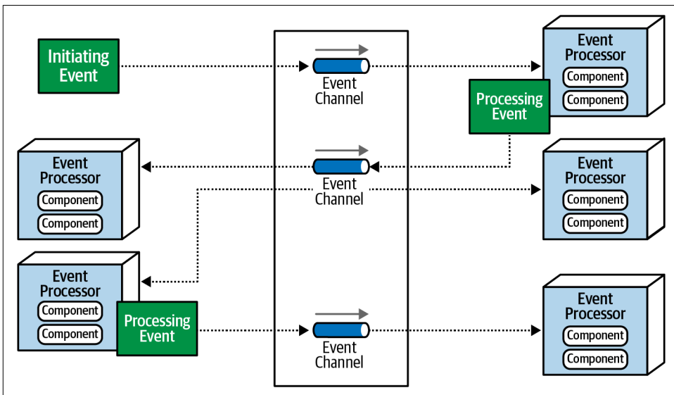
Figure 14-2. Broker topology
