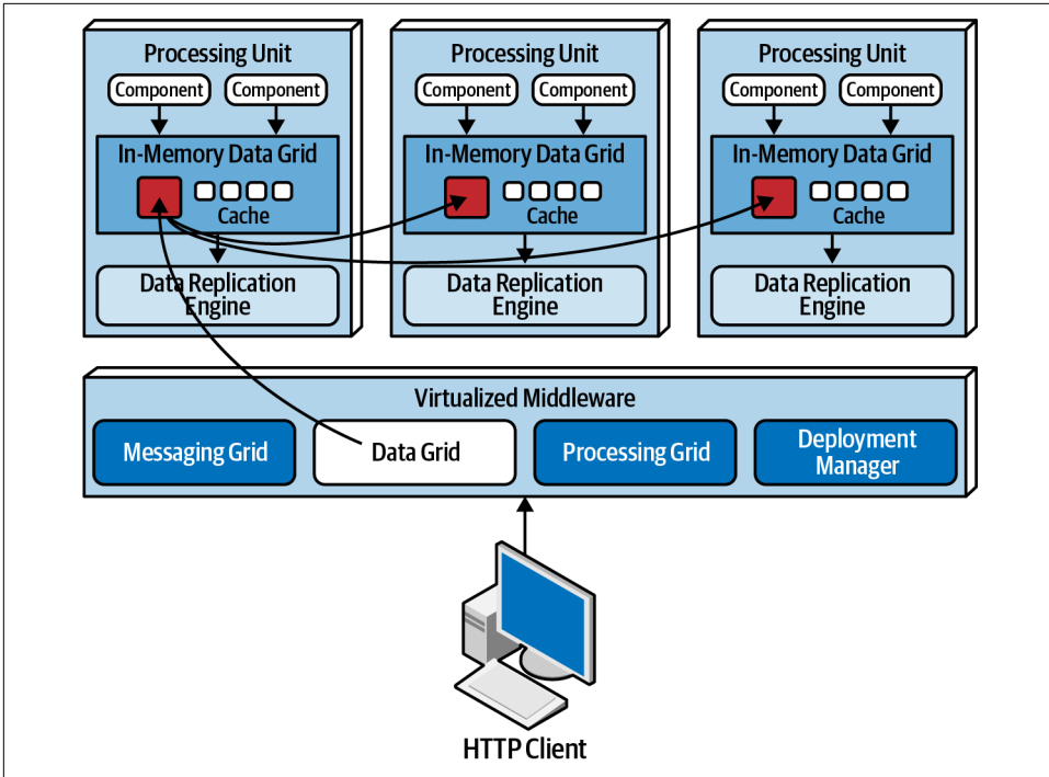
Figure 15-5. Data grid
