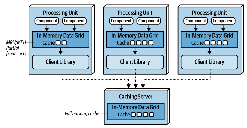
Figure 15-14. Near-cache topology
