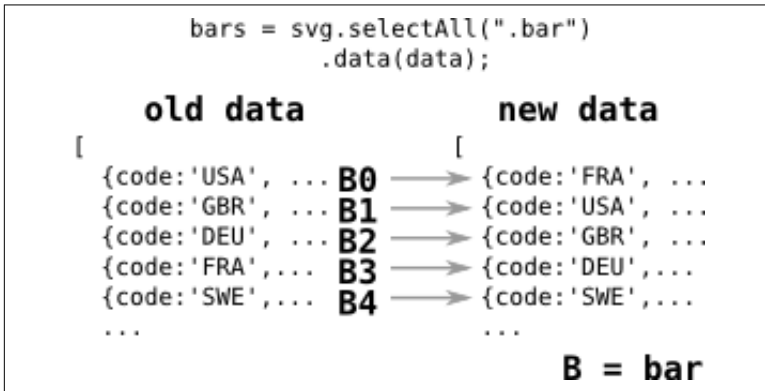
Figure 16-25. By default, new data is joined by index
