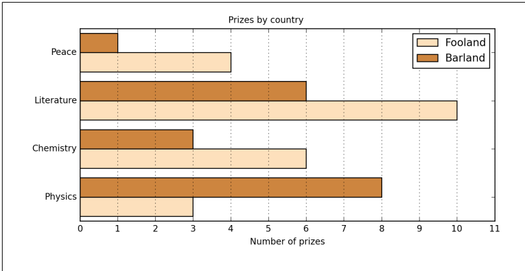
Figure 10-7. Turning the bars on their side
