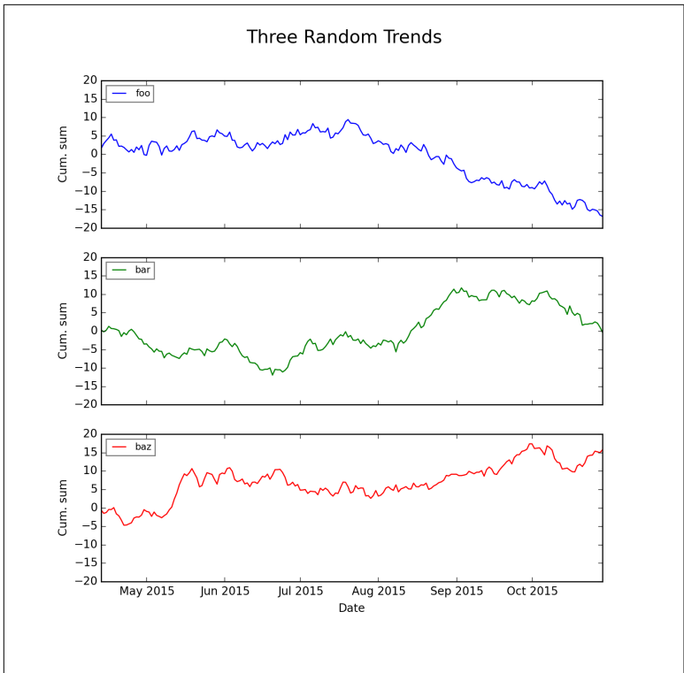
Figure 10-4. Three subplots
