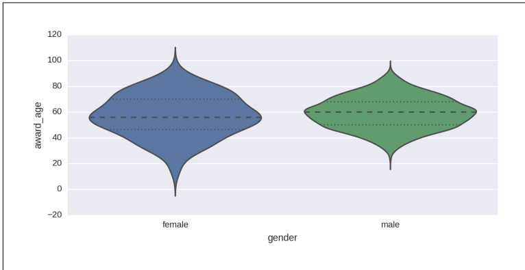
Figure 11-20. Violinplots of prize-age distribution by gender
