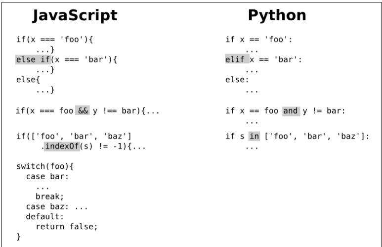
Figure 2-5. Conditionals
