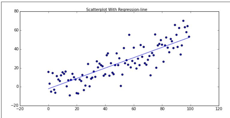
Figure 10-11. Scatter plot with regression line
