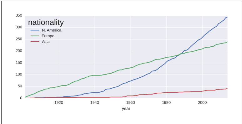
Figure 11-14. Historical prize trends by region
