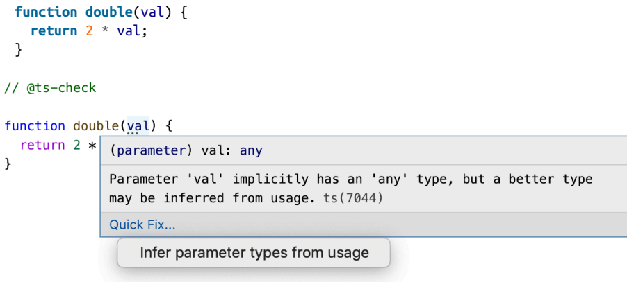
Figure 8-2. The TypeScript Language Services offer a quick fix to infer parameter types from usage.
