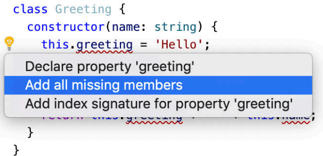
Figure 8-4. The quick fix to add declarations for missing members is particularly helpful in converting a class to TypeScript.
