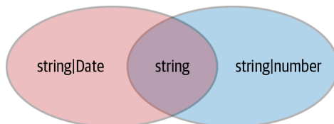
Figure 2-8. Union types may not fit into a hierarchy but can be thought of in terms of sets of values.
