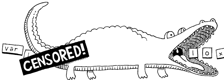
Lexical analyzer.
