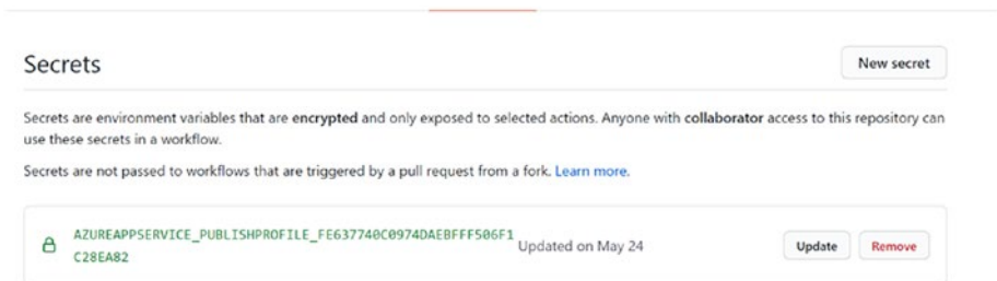
Figure 4-2. New secret
