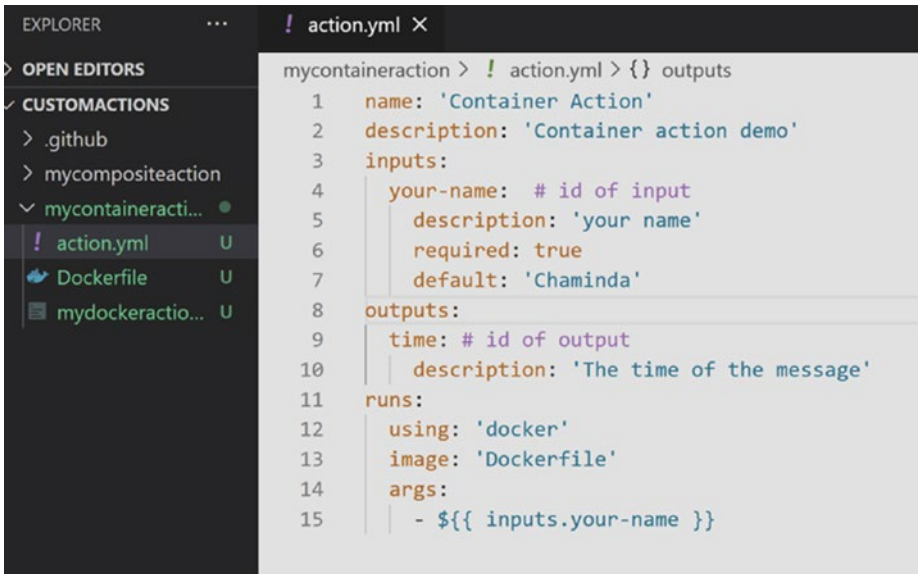
Figure 9-21. Metadata file
