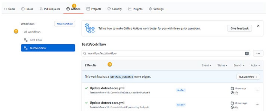
Figure 2-7. Workflow runs
