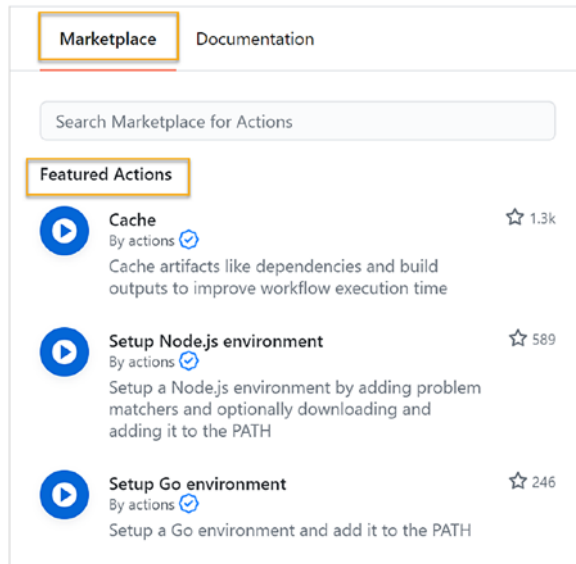
Figure 2-3. Marketplace actions
