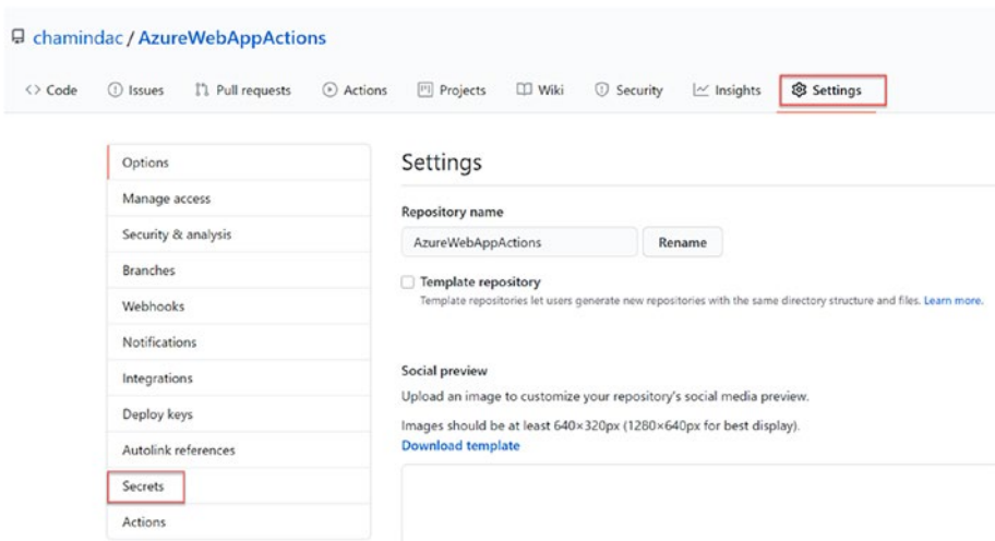
Figure 4-1. Secrets
