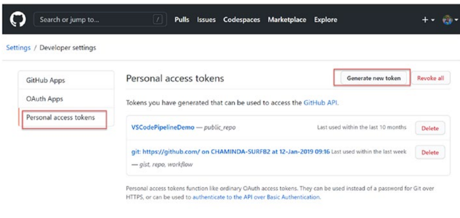
Figure 7-11. Generate token
