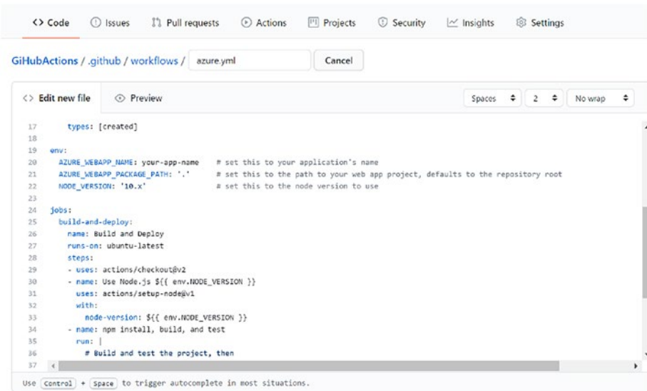
Figure 2-2. Workflow template YAML file
