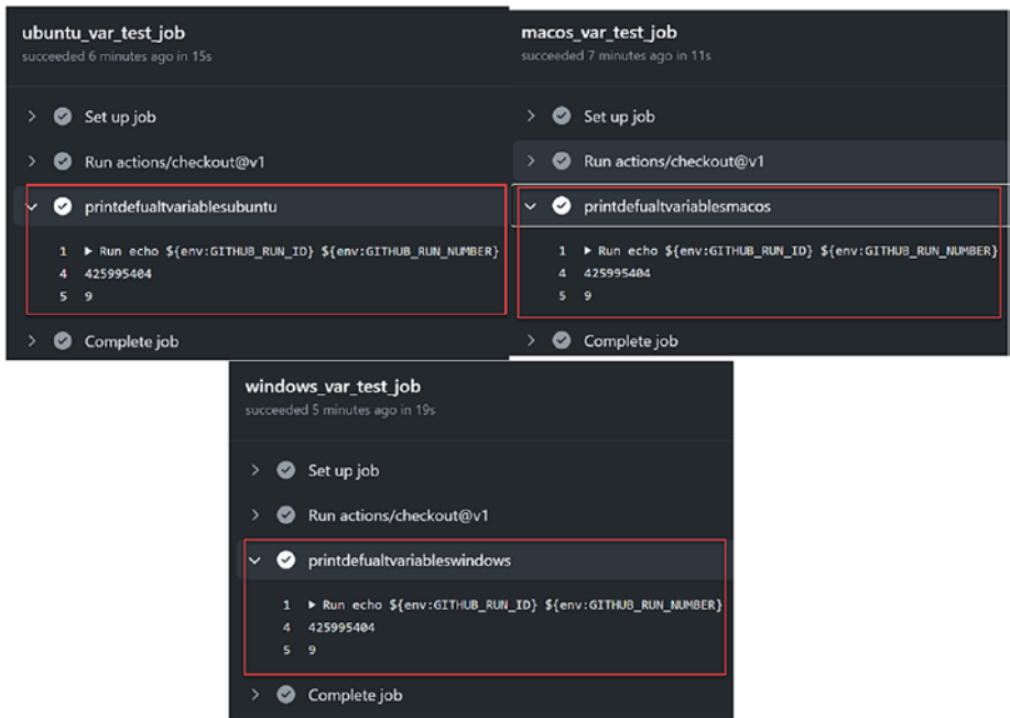
Figure 10-8. \${env.varname} works for PowerShell Core
