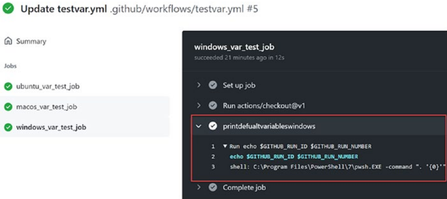
Figure 10-3. Default variables not printed in Windows
