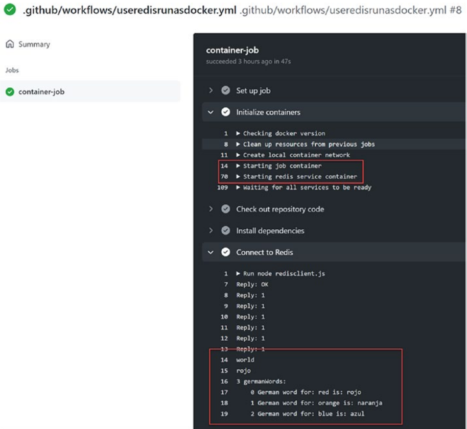
Figure 8-3. Workflow run as container and using Redis service container
