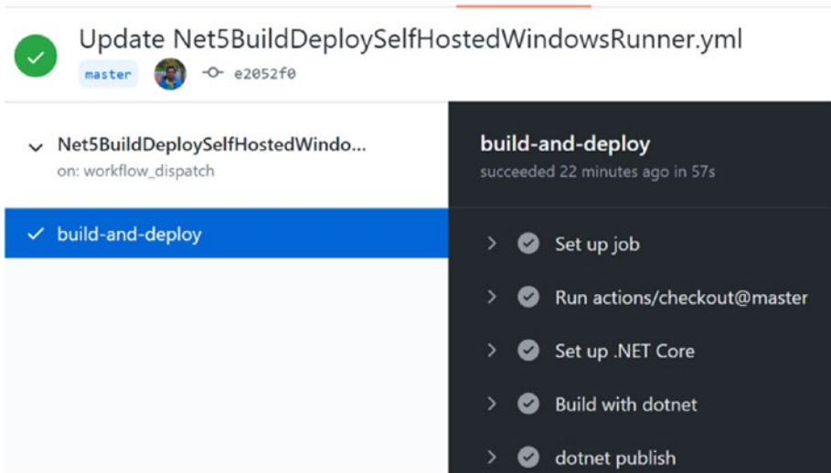
Figure 6-11. Workflow in the self-hosted runner
