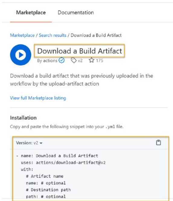
Figure 2-4. Marketplace action YAML script
