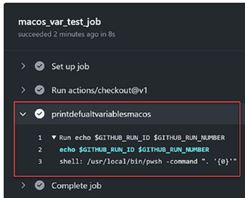
Figure 10-6. PowerShell Core not printing default variables in macOS
