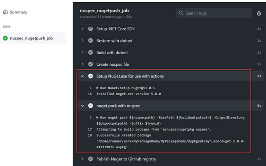
Figure 7-8. Create NuGet package
