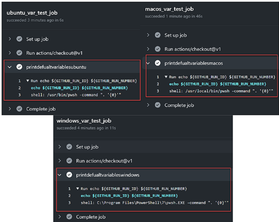
Figure 10-7. ${varname} is not working
