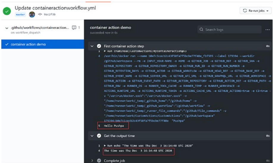
Figure 9-22. Container action used in workflow
