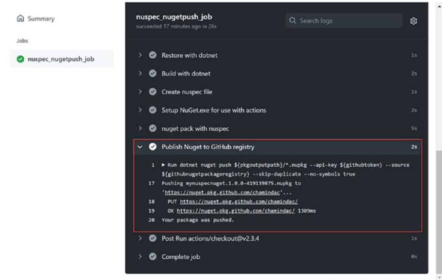
Figure 7-9. Push the package to GitHub Packages
