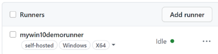
Figure 6-7. Self-hosted runner
