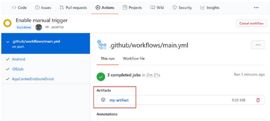
Figure 5-1. Artifacts
