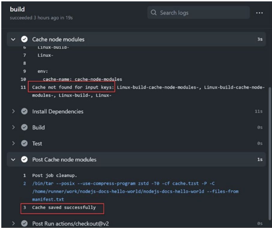
Figure 5-3. Cache node modules
