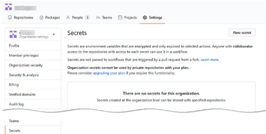
Figure 4-3. Secrets in GitHub organizations
