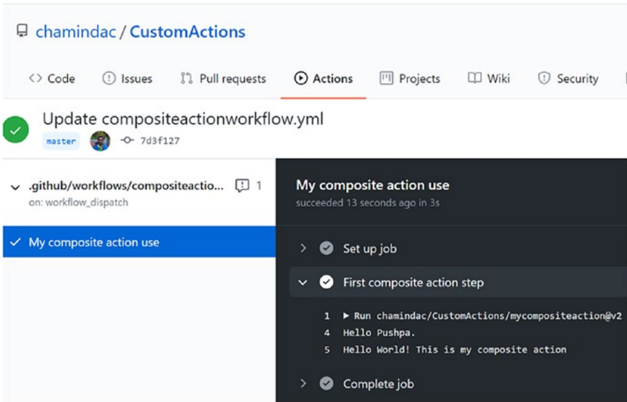
Figure 9-17. Composite action in a workflow
