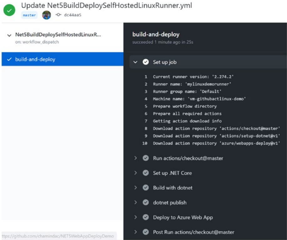
Figure 6-19. Running a workflow on self-hosted Linux runner
