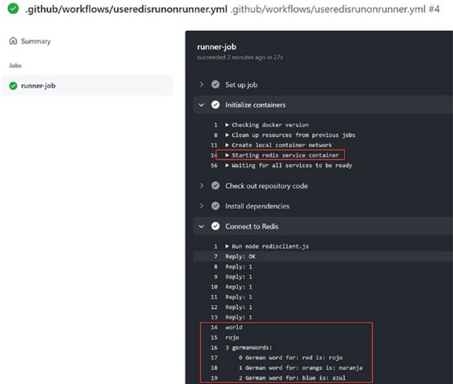
Figure 8-4. Using Redis service container while running job on runner machine
