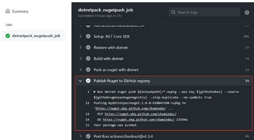
Figure 7-4. Package pushed
