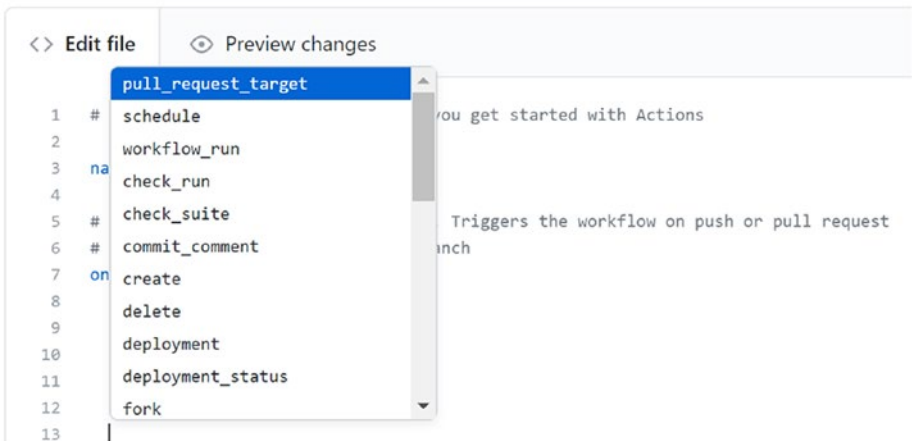
Figure 2-10. Workflow triggers
