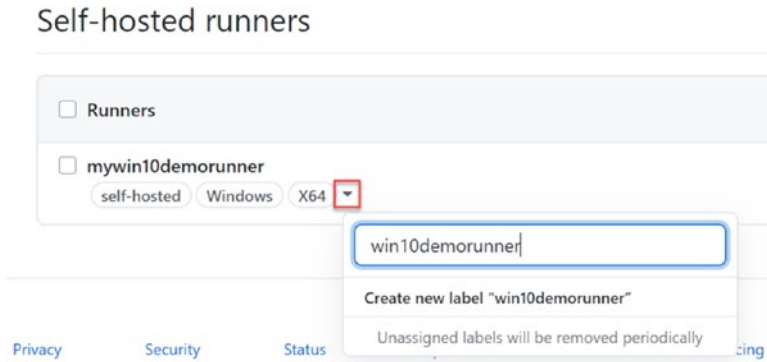
Figure 6-8. Add label
