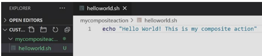
Figure 9-14. helloworld.sh
