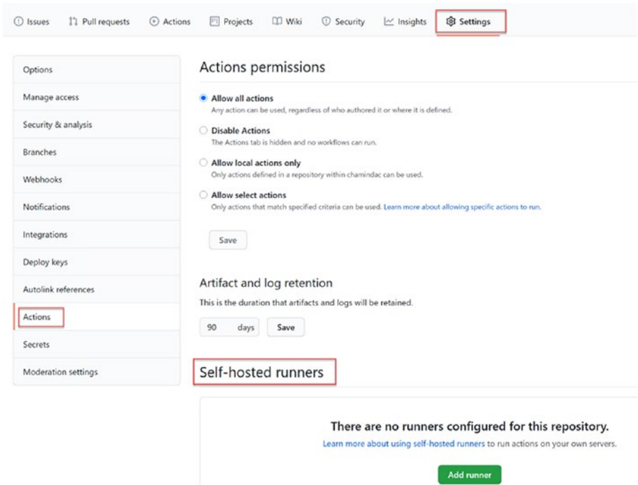
Figure 6-1. Add runner
