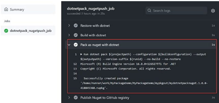
Figure 7-3. dotnet pack
