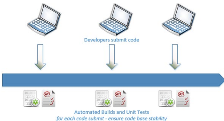
Figure 1-1. Continuous integration
