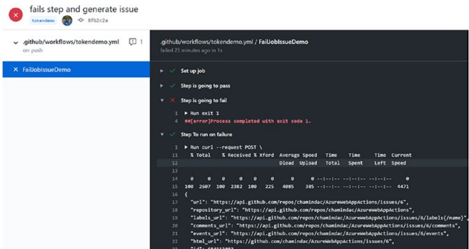
Figure 4-4. Generate issue on failure
