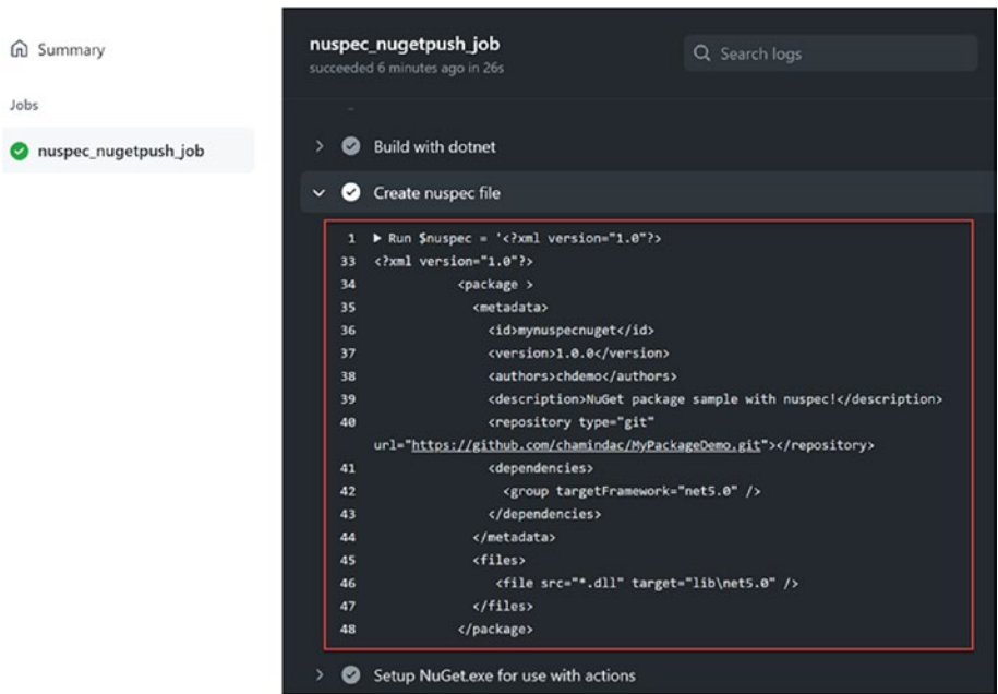
Figure 7-7. Create nuspec in the workflow
