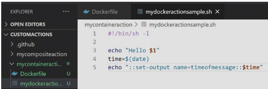
Figure 9-20. Action code to execute in container
