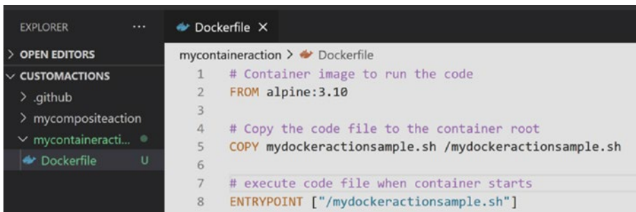
Figure 9-19. Dockerfile
