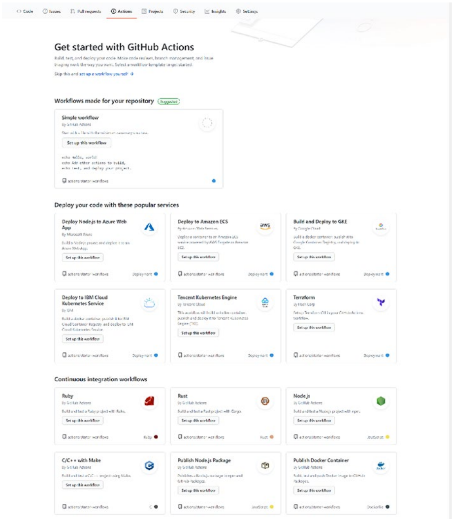
Figure 2-1. Workflow templates
