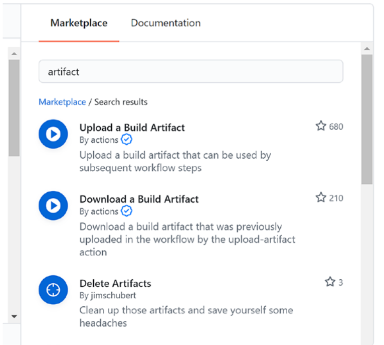
Figure 5-2. Artifact actions
