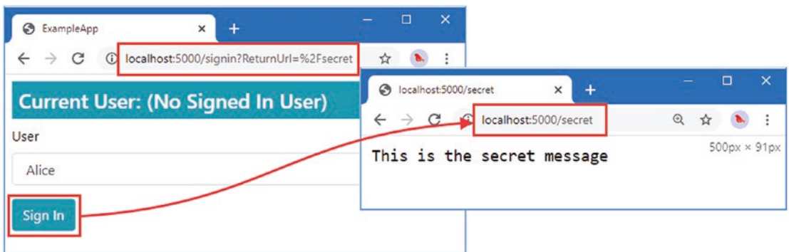
Figure 14-12. Using the ASP.NET Core cookie authentication handler
