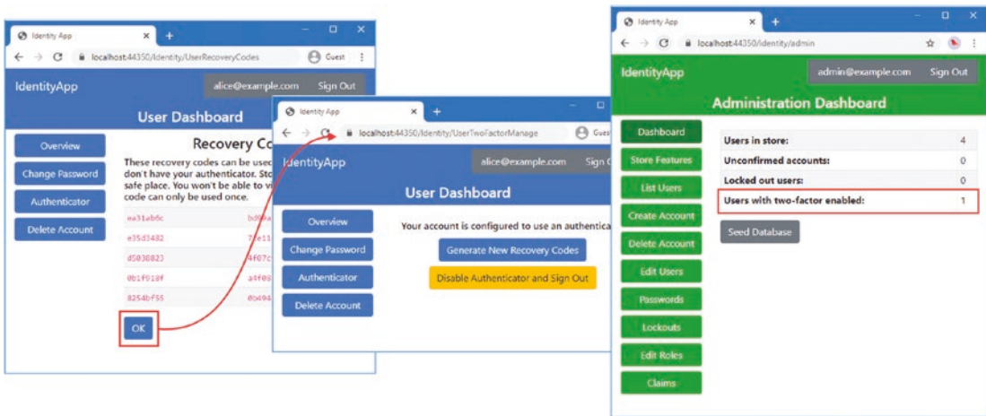
Figure 11-4. Completing the authenticator setup
