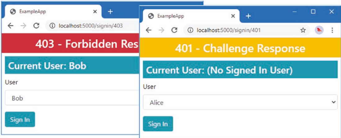
Figure 14-11. Generating HTML responses
