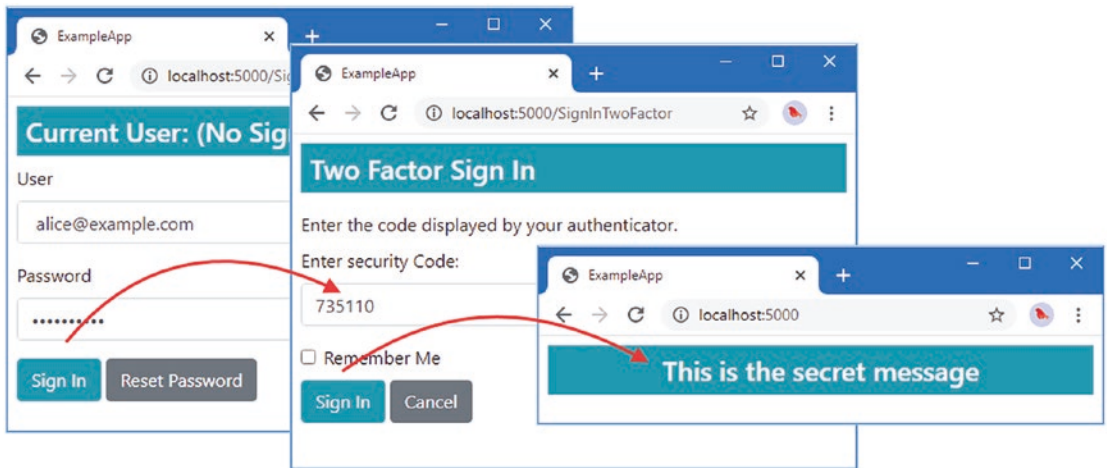
Figure 21-4. Signing in with an authenticator
