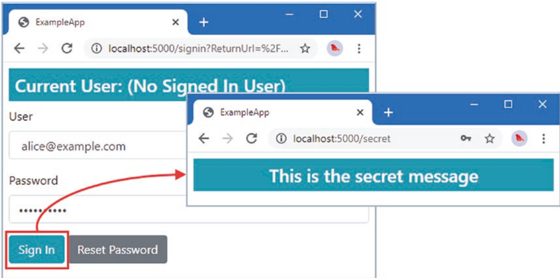
Figure 20-7. The sign-in process with a remembered client
