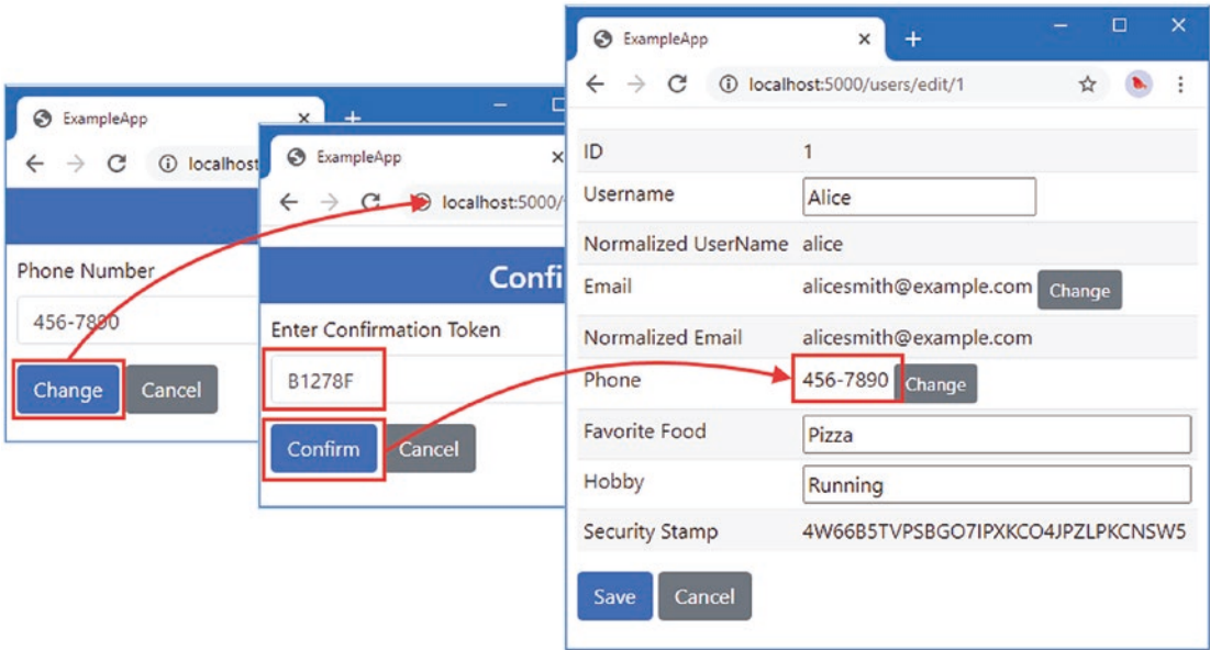
Figure 17-8. Changing a phone number
