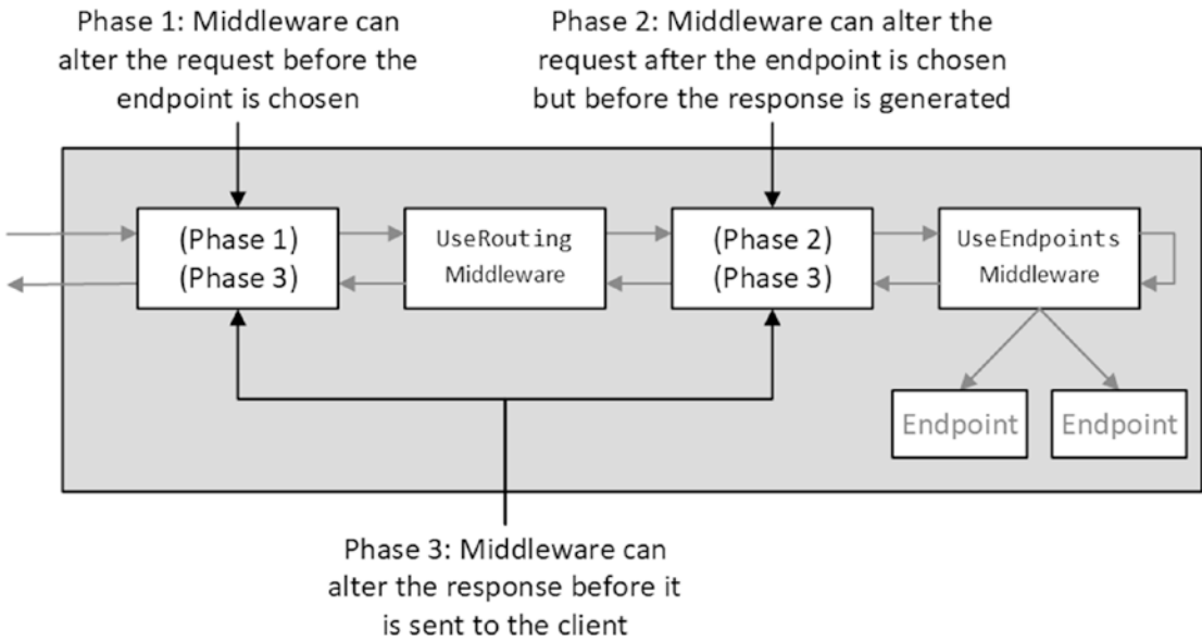
Figure 14-3. The effect of endpoint routing on the request pipeline
