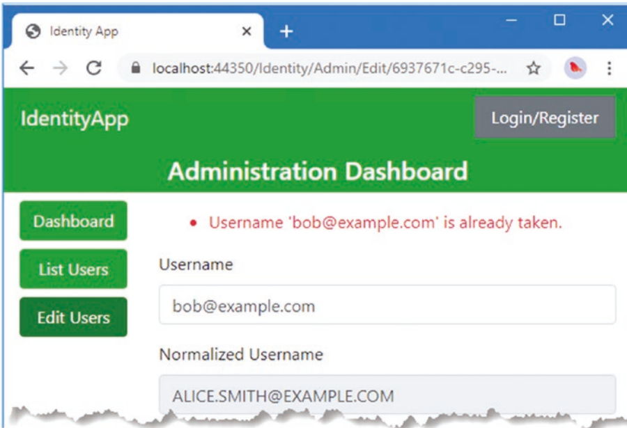
Figure 7-8. Validating user details
