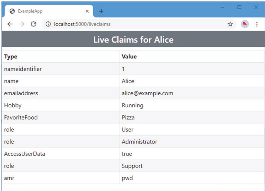
Figure 19-7. Claims derived from roles
