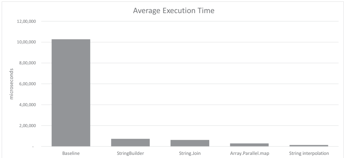
Figure 12-4. Impact of various improvements to string building
