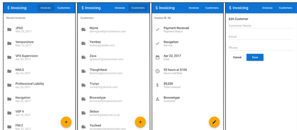
Figure 9.2 Invoicing application screens, emulated in a mobile device size. From left to right: list of invoices, list of customers, invoice detail view, and customer form.
